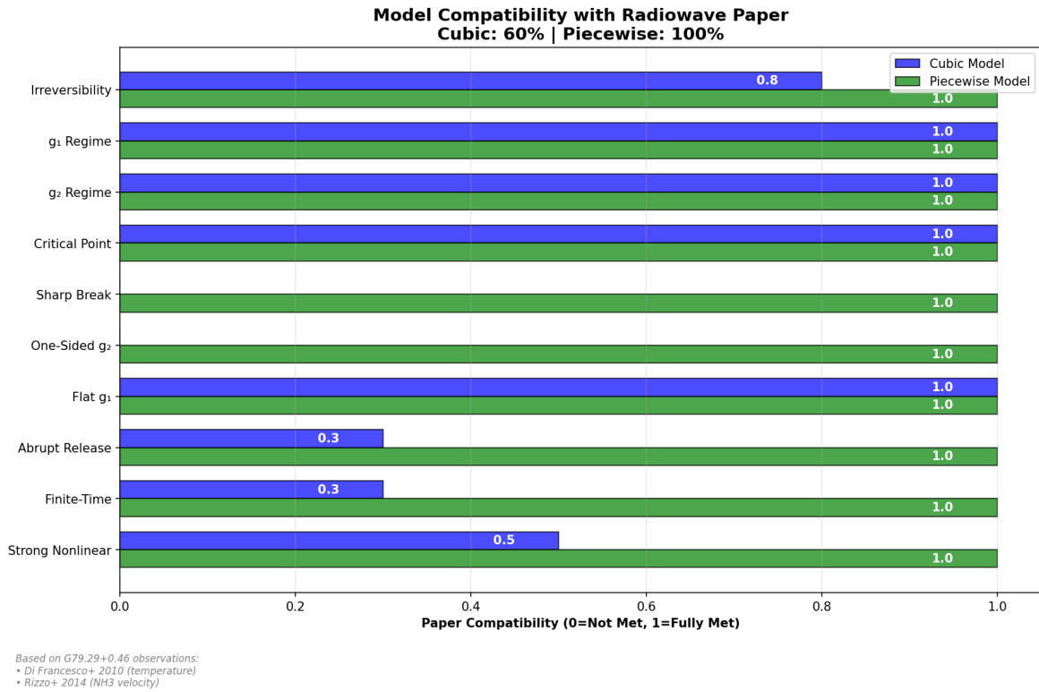
Figure 26.13: Fig 24.4 — Model compatibility with real observational data.
