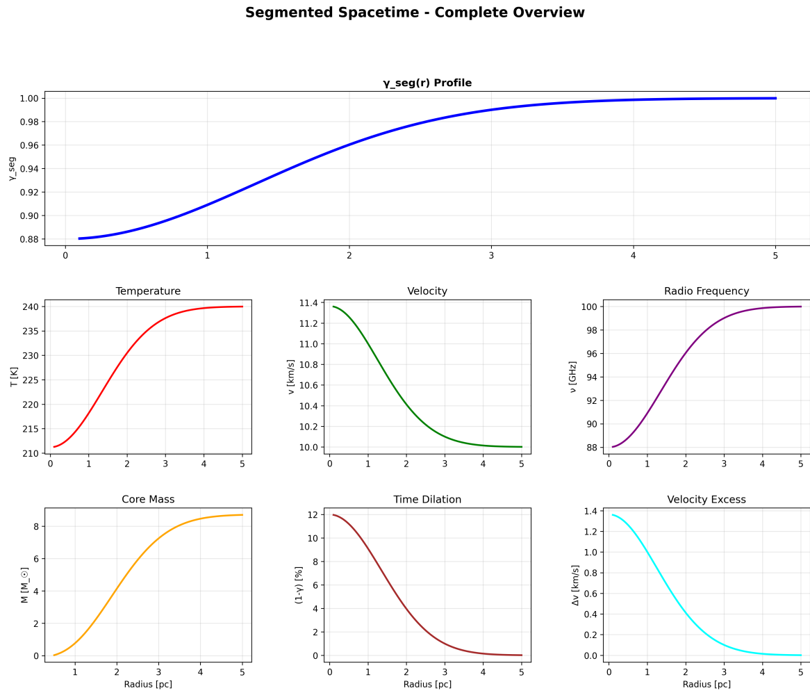
Figure 26.10: Fig 24.1 — G79 Summary Dashboard.
