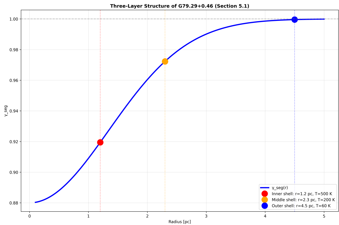
Figure 26.11: Fig 24.2 — G79 Multi-Shell Structure.
