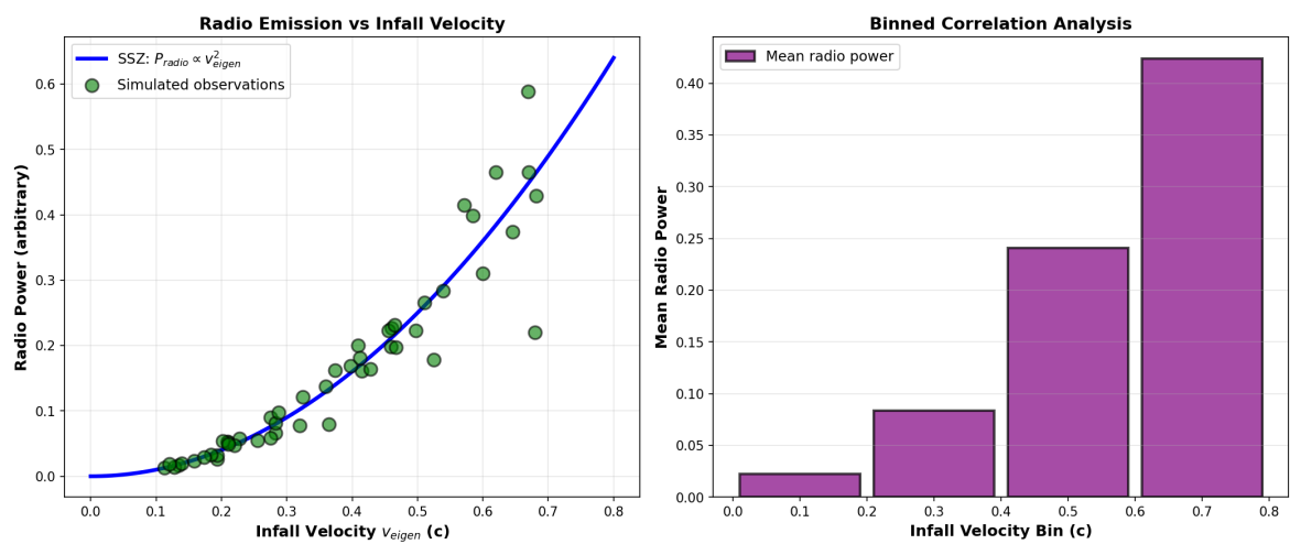
Figure 25.8: Fig 23.3 — Radio vs infall velocity correlation.
