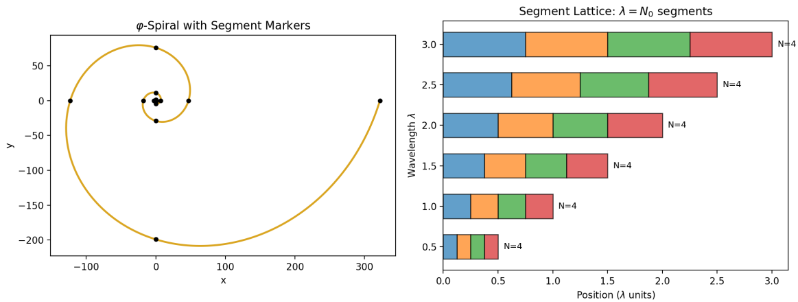
Figure 2.1: Fig 2.1 — Structural Constants: \phi -spiral with segment markers (left) and segment lattice \lambda = N_0 segments (right).
