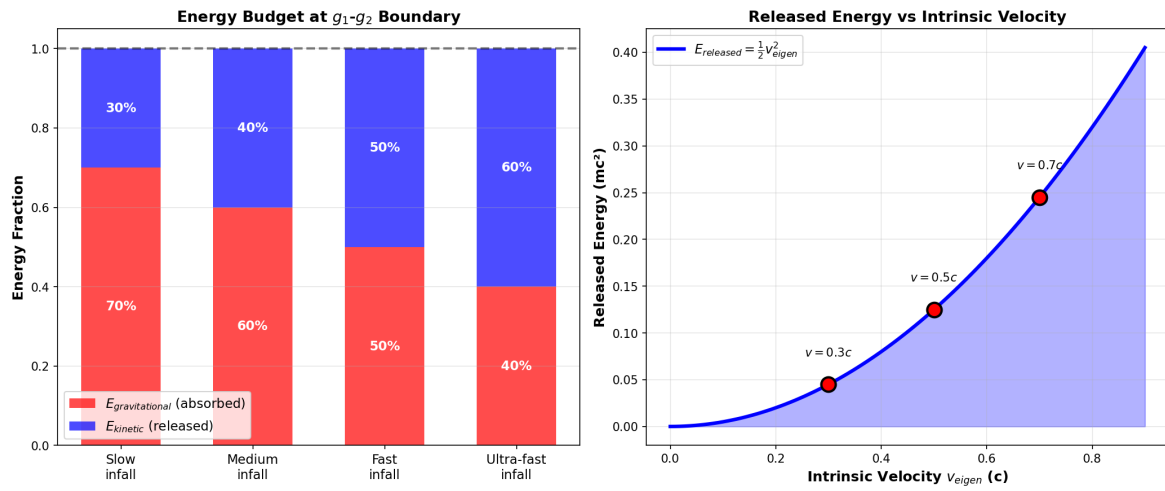
Figure 25.9: Fig 23.4 — Energy budget conservation in SSZ infall.
