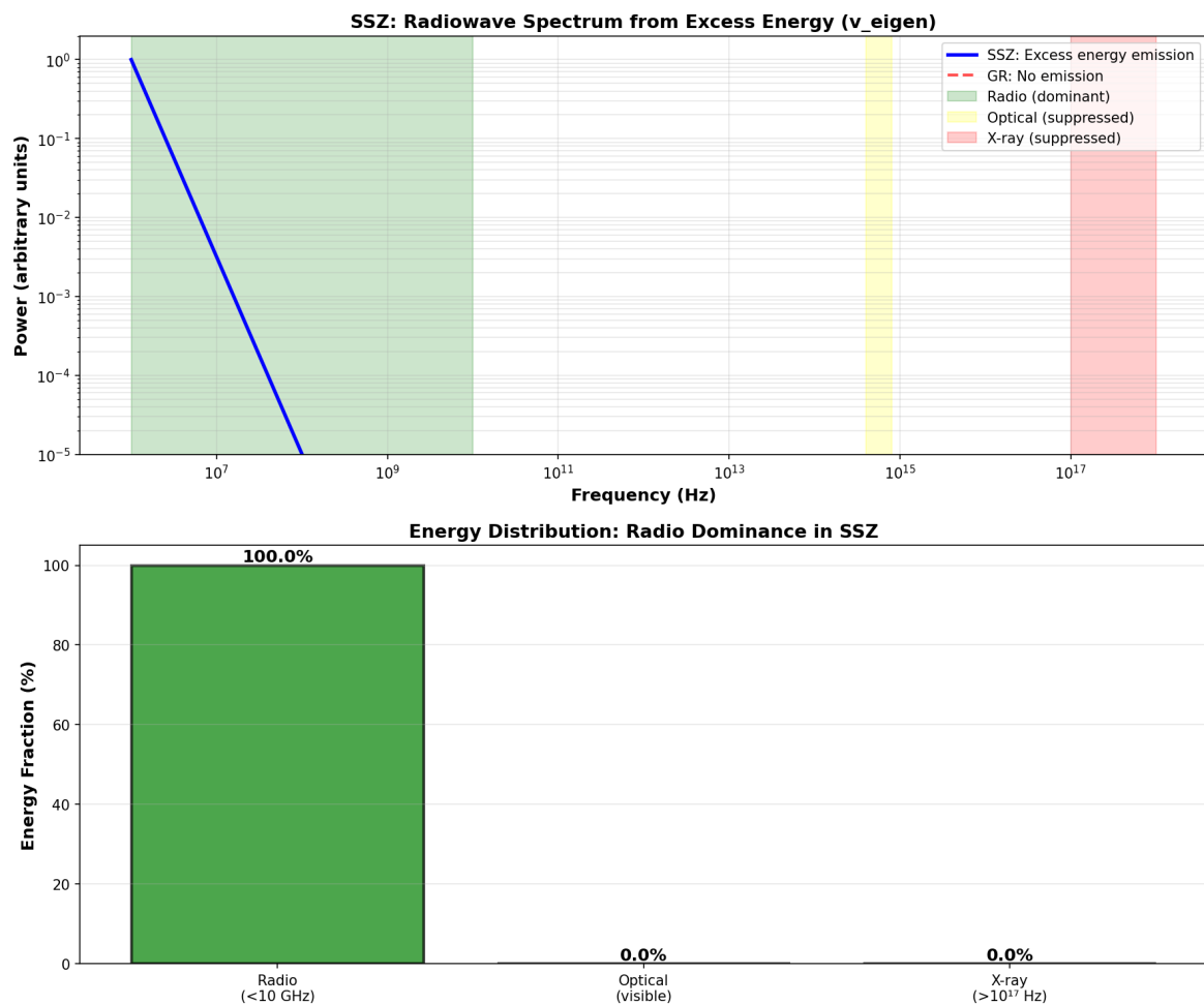
Figure 25.6: Fig 23.1 — Radiowave spectrum: Excess energy from segment-based propagation.
