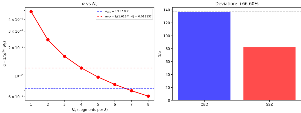
Figure 5.1: Fig 5.1 — Geometric Origin of \alpha : \alpha = 1/(\phi^{2n} \cdot N_0) as function of N_0 (left) and comparison with QED value (right).
