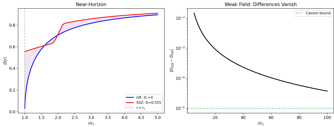
Figure 1.2: Fig 1.2 — GR vs SSZ: Near-horizon comparison of D(r) (left) and weak-field difference convergence with Cassini bound (right).
