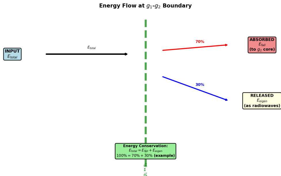
Figure 25.10: Fig 23.5 — Energy flow diagram for infalling matter.
