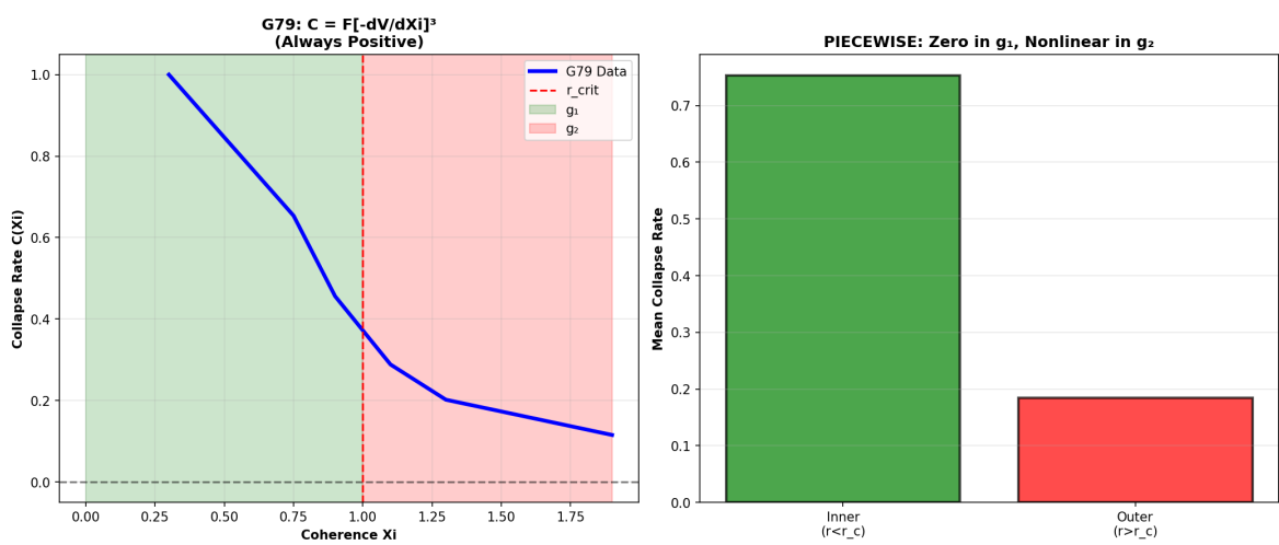
Figure 26.12: Fig 24.3 — Collapse rate from real data.
