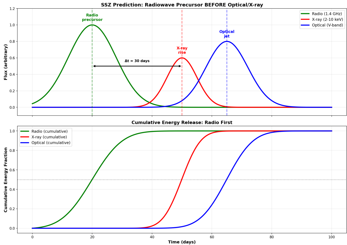
Figure 25.7: Fig 23.2 — Radiowave before optical: Timeline of precursor signal.
