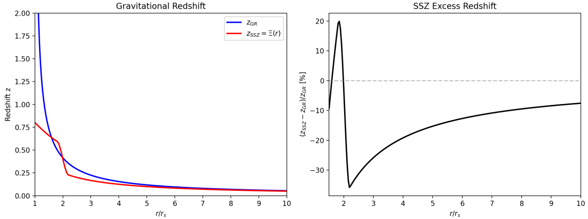
Figure 14.1: Fig 14.1 — Gravitational Redshift: z_{GR} vs z_{SSZ} = \Xi(r) (left) and SSZ excess redshift percentage (right).
