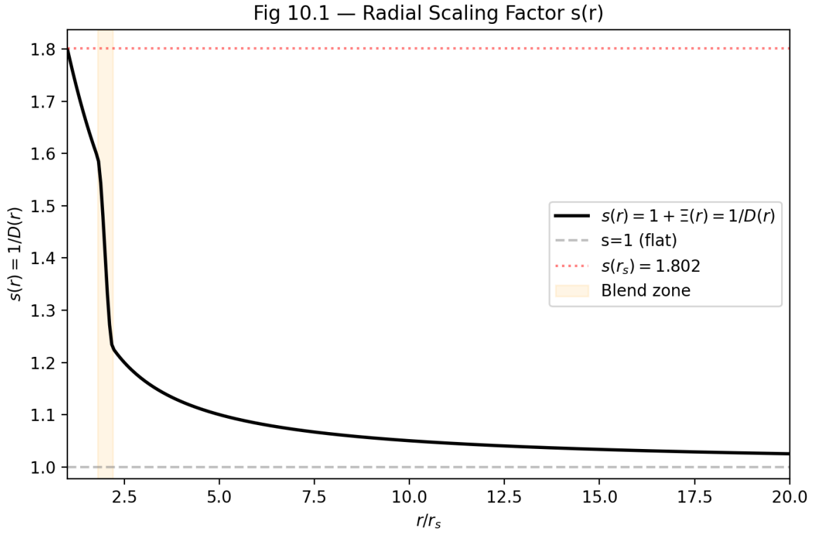
Figure 10.1: Fig 10.1 — Radial Scaling Factor s(r) = 1 + \Xi(r) = 1/D(r) showing the blend zone and saturation at s(r_s) = 1.802 .
