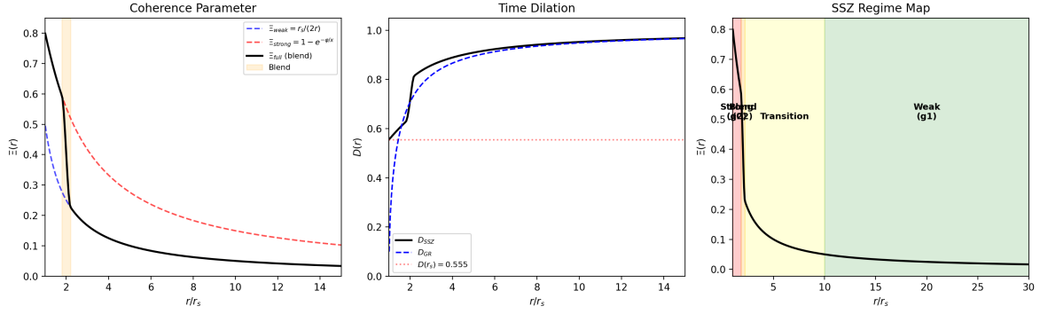
Figure 1.1: Fig 1.1 — SSZ Overview: Coherence parameter \Xi(r) , time dilation D(r) , and regime map showing weak ( g_1 ), transition, and strong ( g_2 ) regions.
