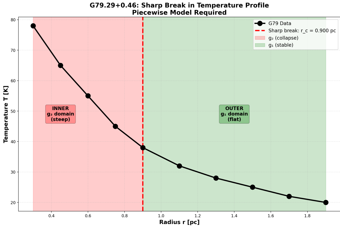
Figure 27.14: Fig 25.1 — Temperature profile with sharp break at the g_2 \rightarrow g_1 transition.
