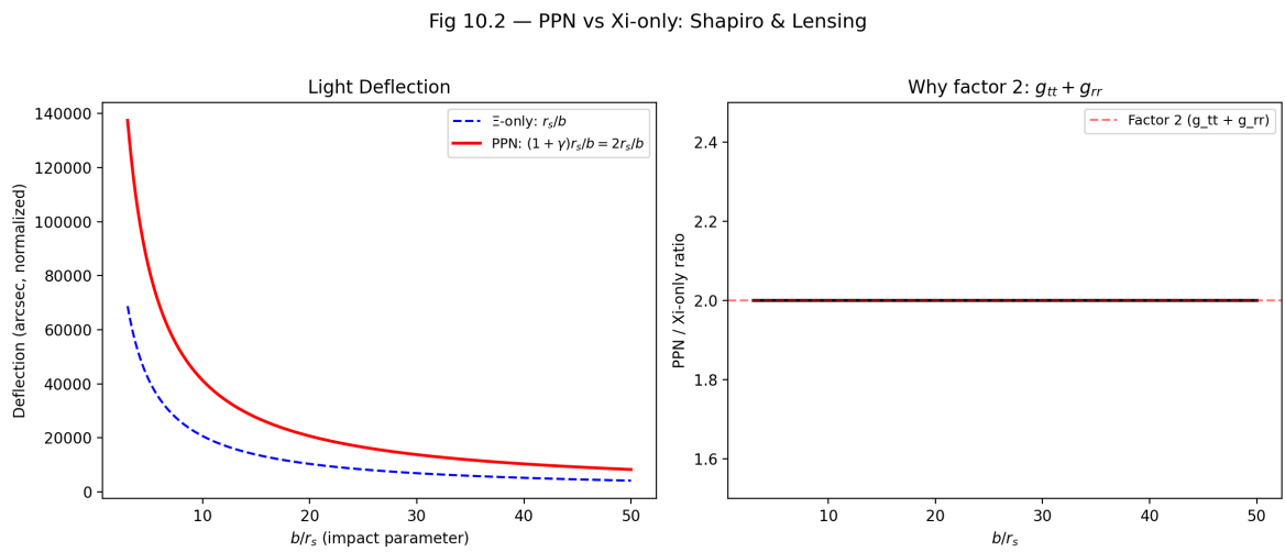
Figure 10.2: Fig 10.2 — PPN vs \Xi -only: Light deflection (left) and the factor-2 ratio g_{tt} + g_{rr} (right) confirming (1+\gamma) = 2 .
