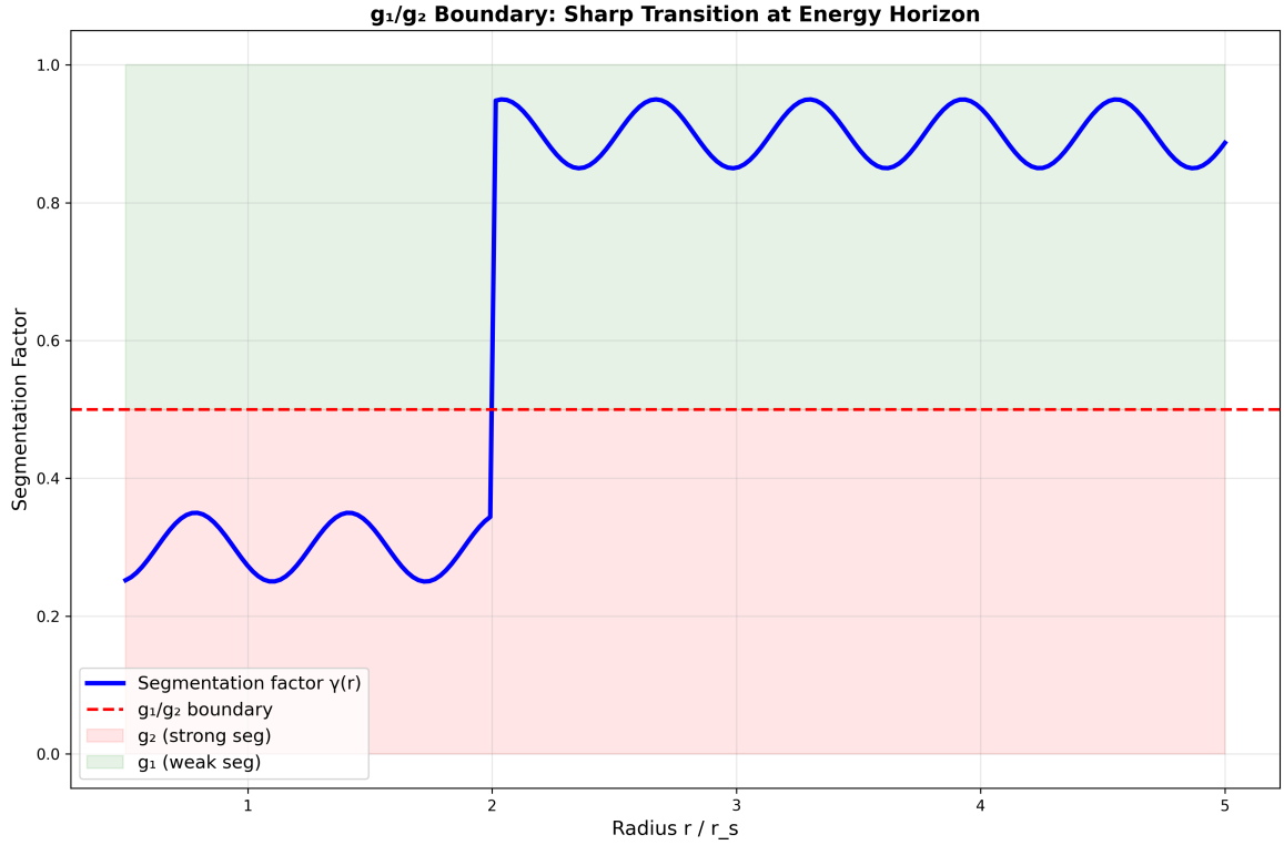
Figure 25.11: Fig 23.6 — g_1/g_2 boundary physics and observational predictions.
