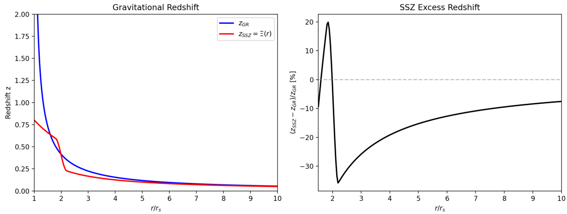
Figure 14.1: Fig 14.1 — Gravitational Redshift: z_{GR} vs z_{SSZ} = \Xi(r) (left) and SSZ excess redshift percentage (right).
