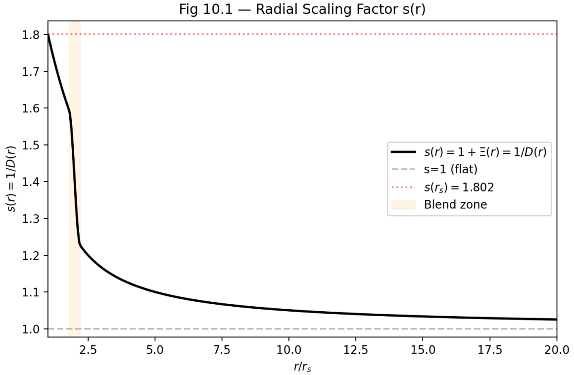
Figure 10.1: Fig 10.1 — Radial Scaling Factor s(r) = 1 + \Xi(r) = 1/D(r) showing the blend zone and saturation at s(r_s) = 1.802 .
