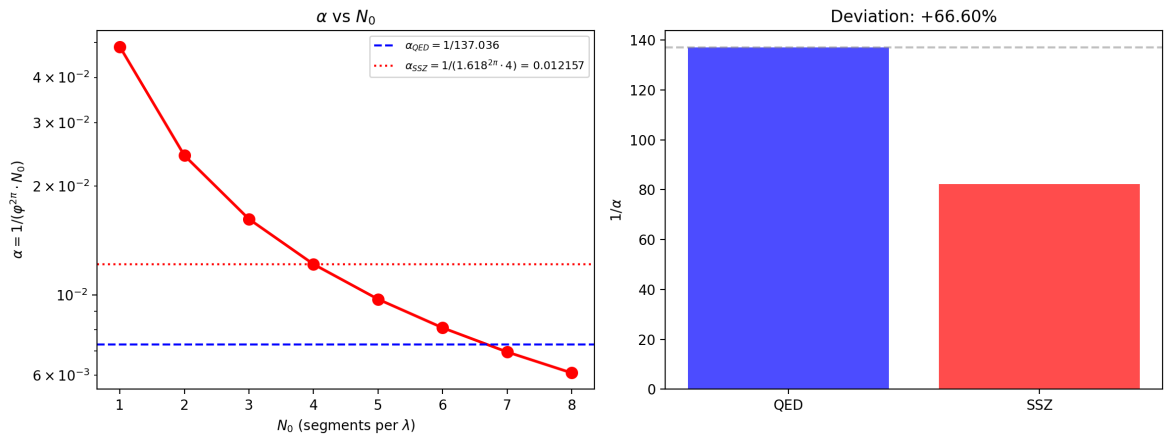
Figure 5.1: Fig 5.1 — Geometric Origin of \alpha : \alpha = 1/(\varphi^{2n} \cdot N_0) as function of N_0 (left) and comparison with QED value (right).
