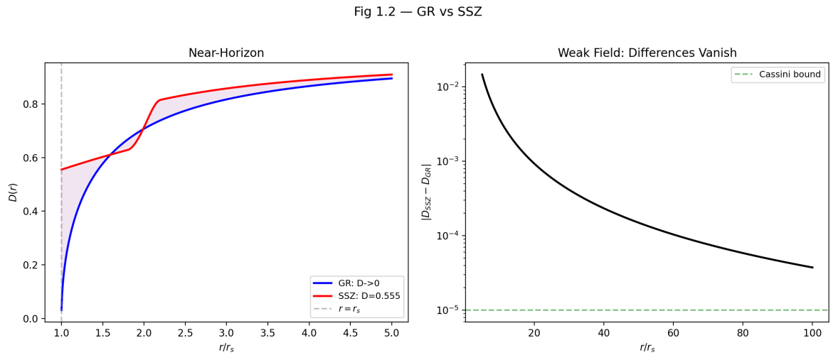
Figure 1.2: Fig 1.2 — GR vs SSZ: Near-horizon comparison of D(r) (left) and weak-field difference convergence with Cassini bound (right).
