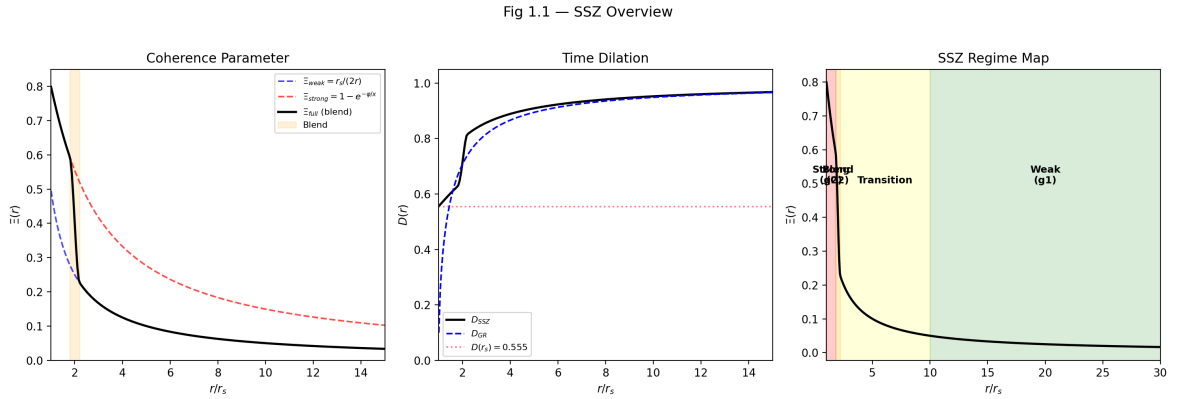
Figure 1.1: Fig 1.1 — SSZ Overview: Coherence parameter \Xi(r) , time dilation D(r) , and regime map showing weak ( g_1 ), transition, and strong ( g_2 ) regions.
